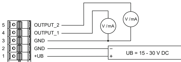
Fig. 2 Voltage supply and outputs
