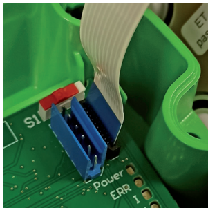
Fig. 8 FFC cable connection on the Sigma 05 electronics board
