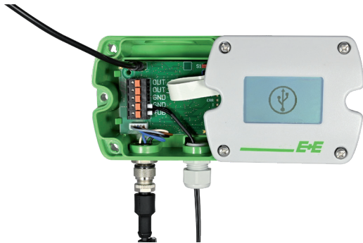
Fig. 6 Sigma 05 with USB connection active only
