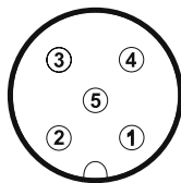
M12 device socket front view
