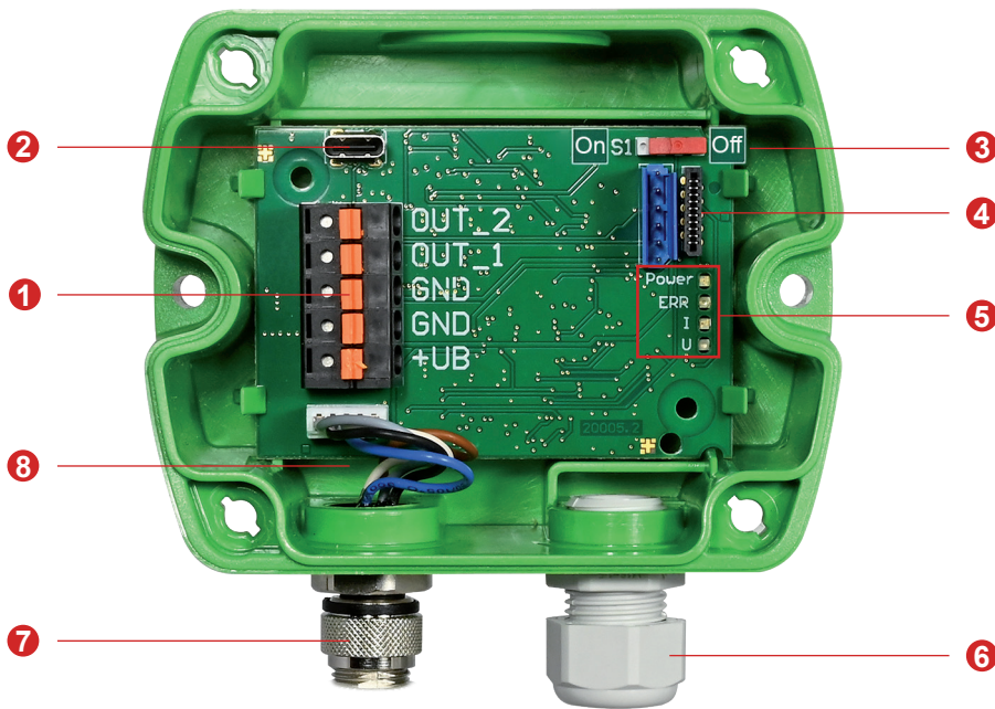
Fig. 3 Sigma 05 electronics board
