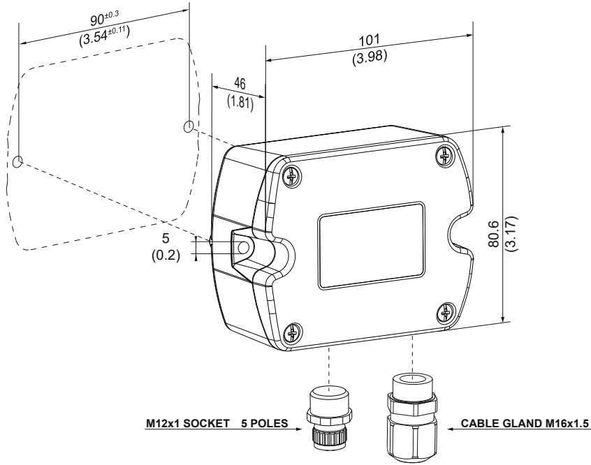
Fig. 1 Sigma 05 dimensions in mm (inch)
